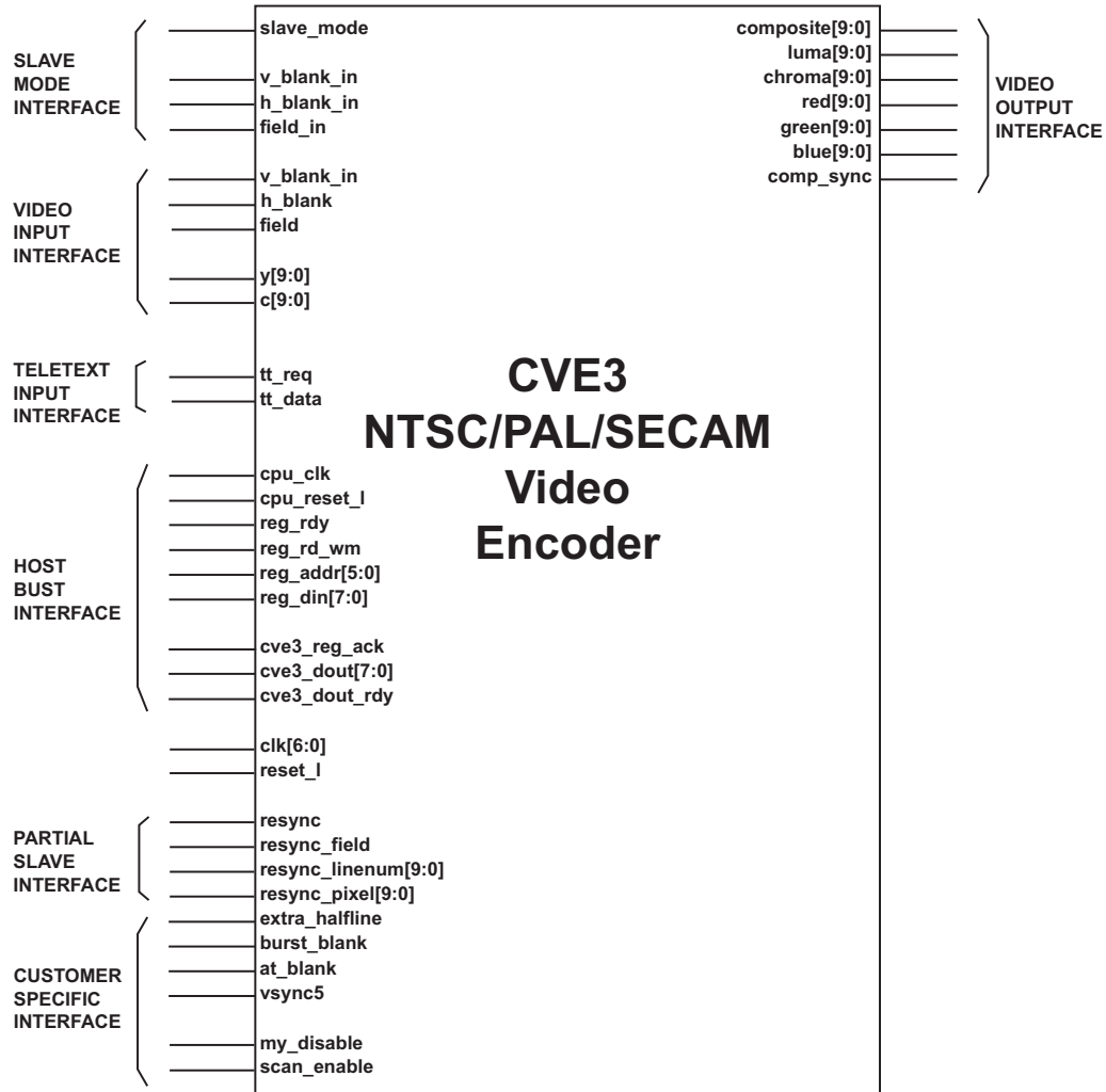
Figure 2. CVE3 Video Encoder Pinout Diagram
